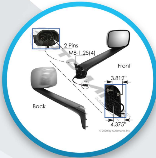
Hood Mount Mirror RH Chrome Freightliner 563.46092C
