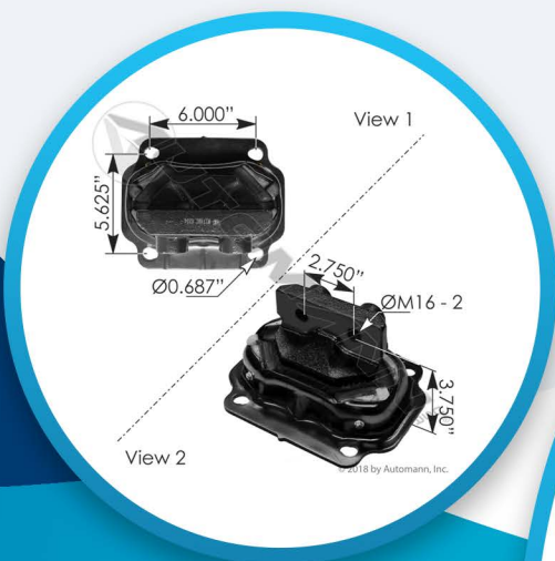
Motor Mount Rear Kenworth M17497
